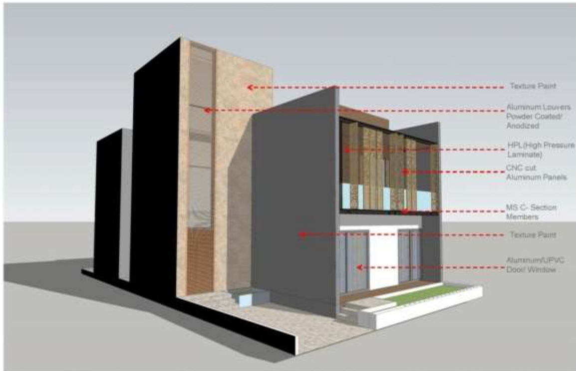
Detailing the exterior with Materials and Texture and treating the balcony projection with CNC cut Aluminium Panels.
