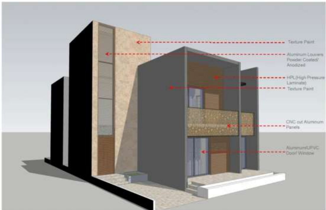
Detailing the exterior with Materials and Texture and treating the openings to balance the vertical and horizontal elements.
